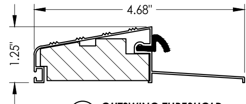
29 OUTSWING THRESHOLD DLP Industries
