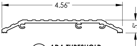
30 ADA THRESHOLD DLP Industries
