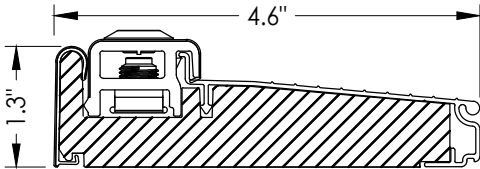
20 INSWING THRESHOLD ENDURA "Z" Series
